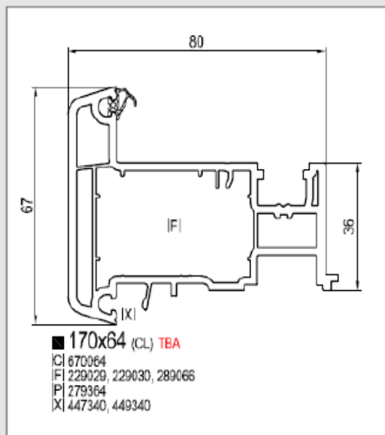
Stulp | 67mm
