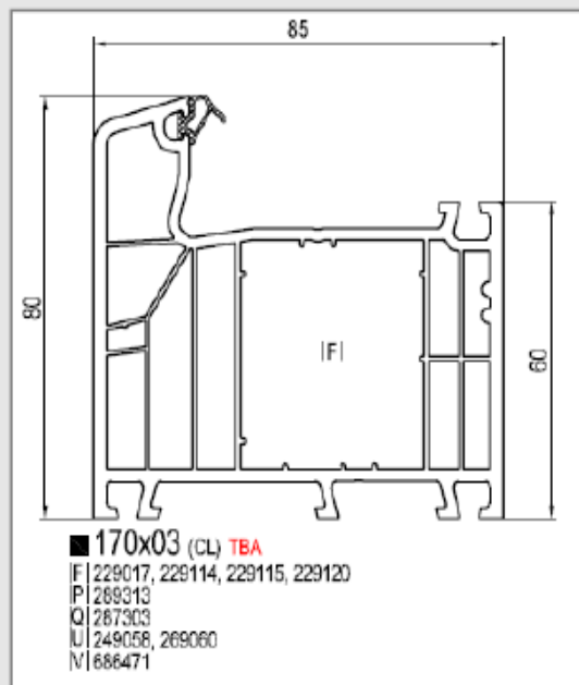
Blendrahmen | 80mm
